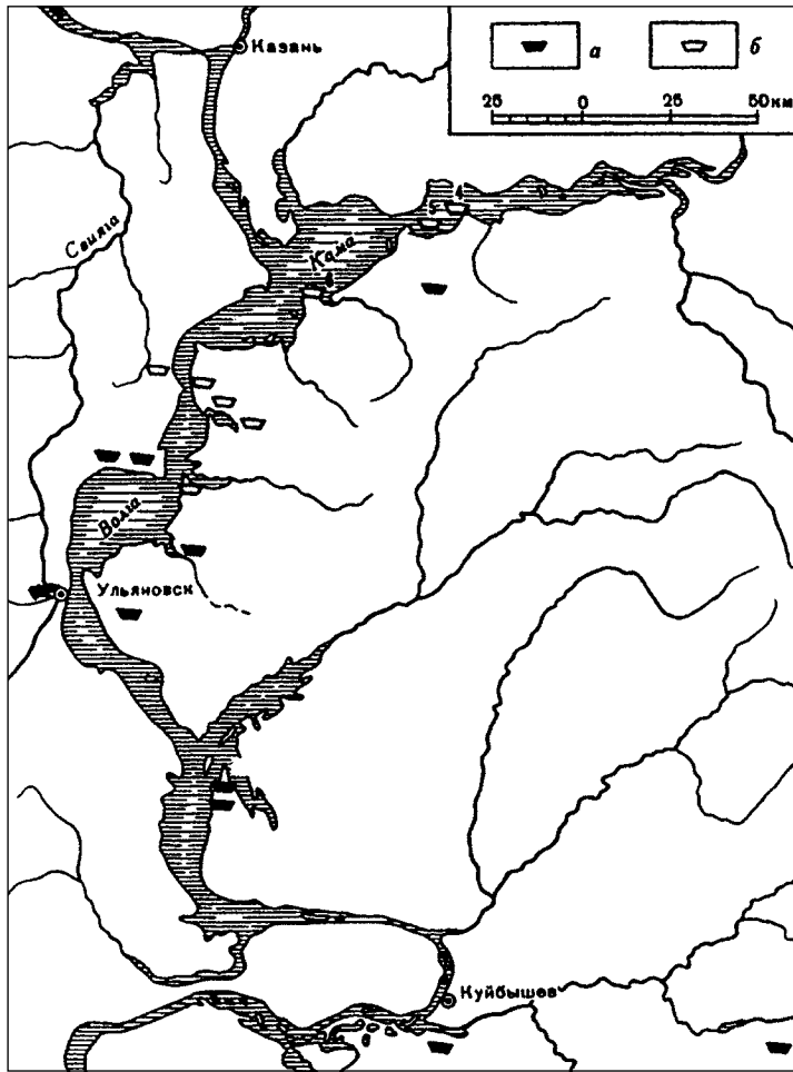
Fig. 1. Cemeteries along the Middle Volga from the 8 th - 10 th c. a) First wave of migrations; б) Second wave of migrations (after Казаков 1992, fig. 1).
